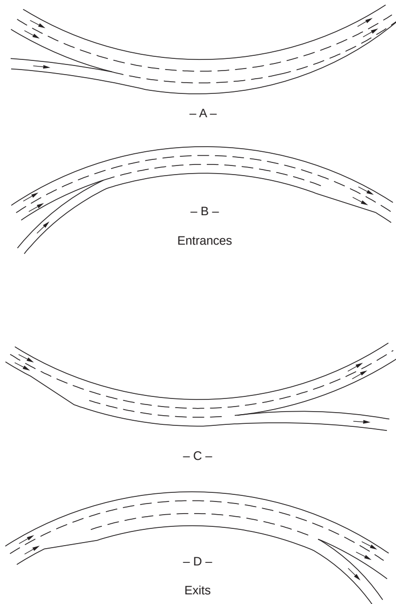
Figure 10-72. Parallel-Type Ramp Terminals on Curves
