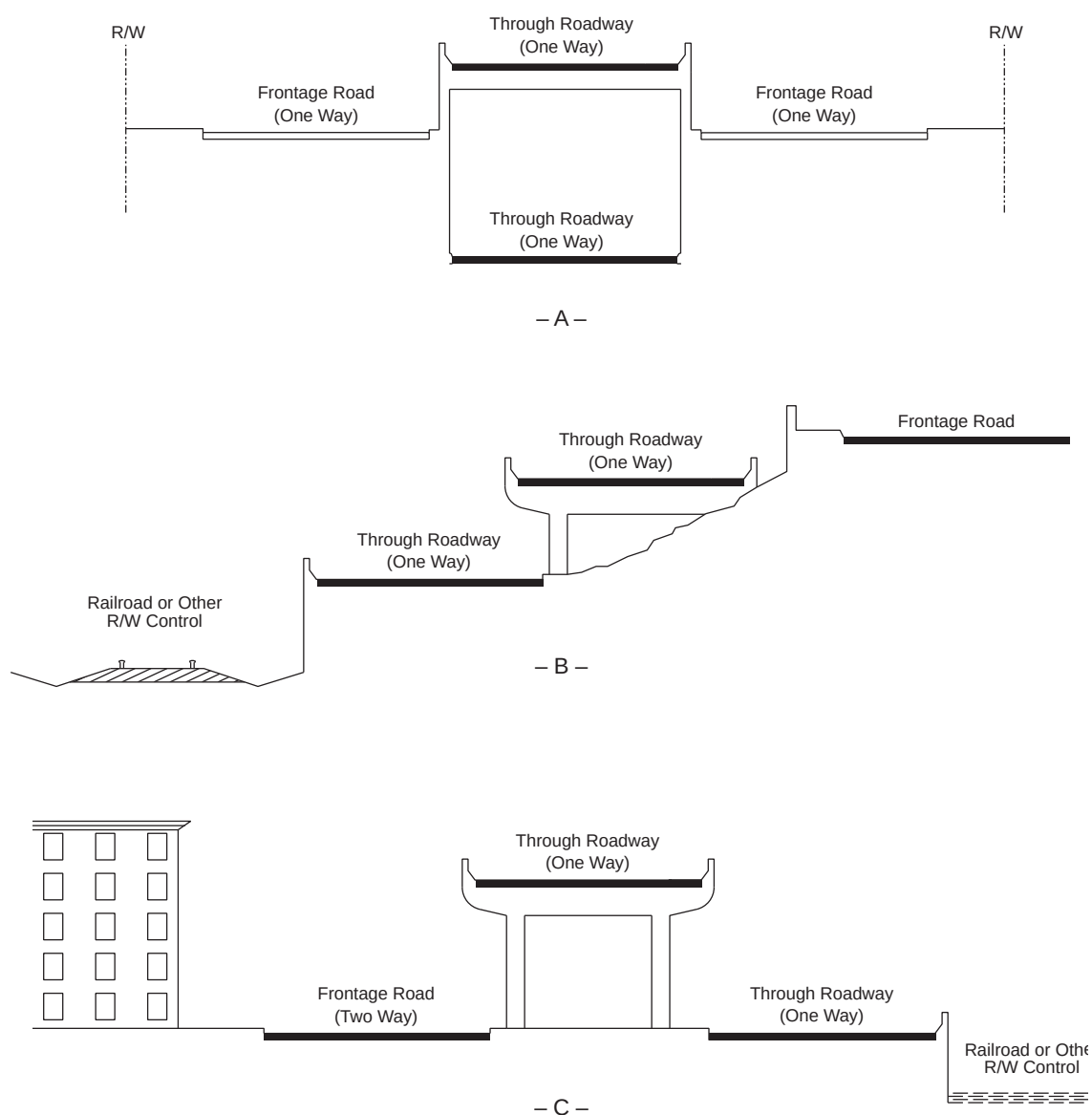
Figure 8-16. Cross-Section Control—Combination-Type Freeway
