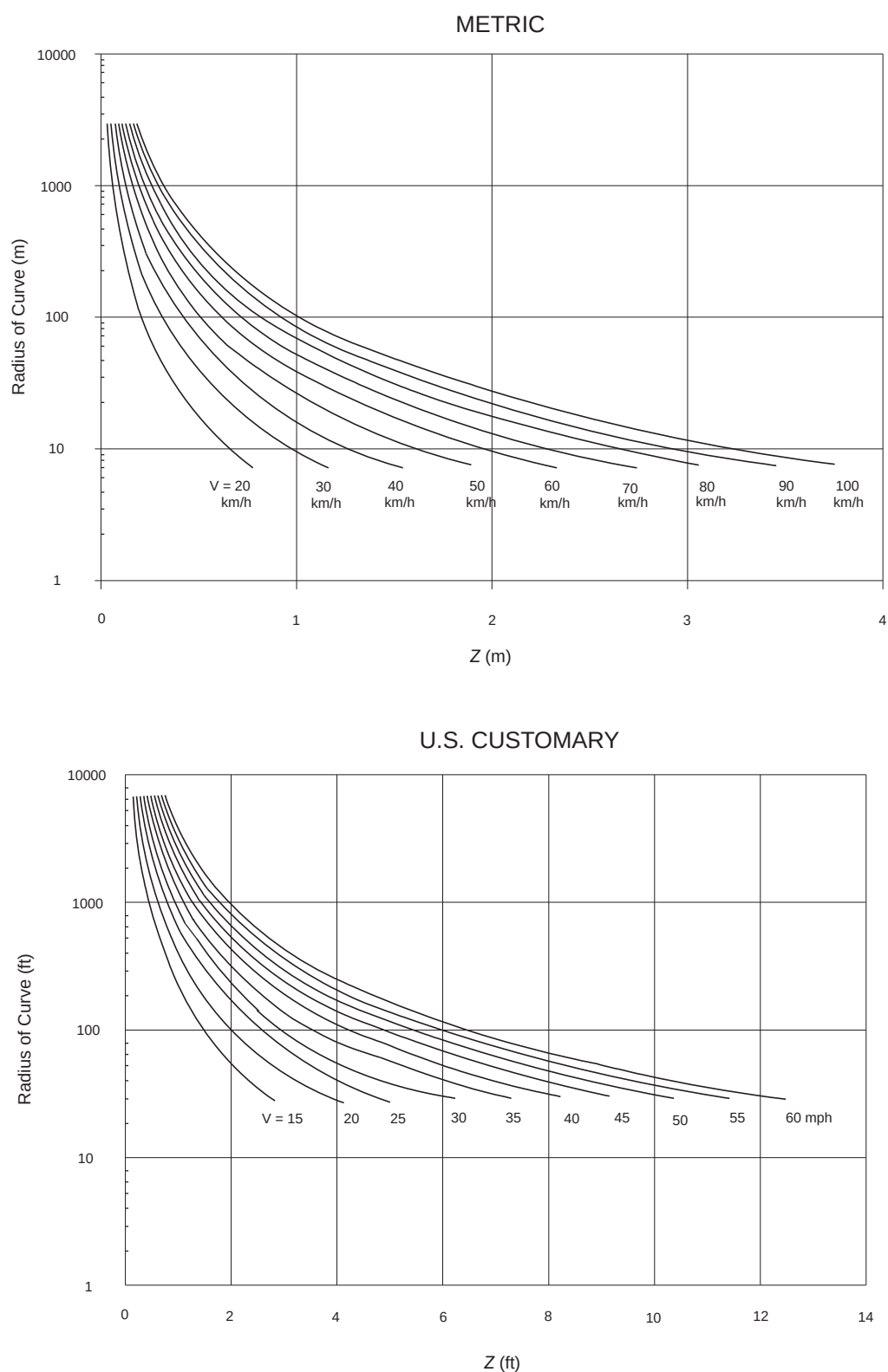
Figure 3-19. Extra Width Allowance for Difficulty of Driving on Traveled Way on Curves
