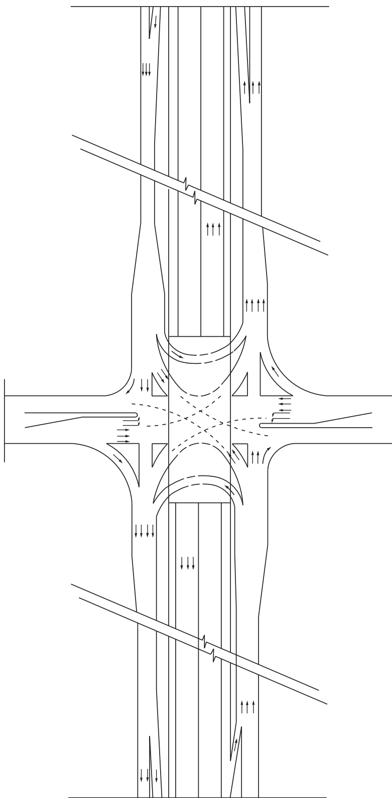
Figure 10-25. Overpass Layout for an SPD with a Frontage Road and a Separate U-Turn Movement
