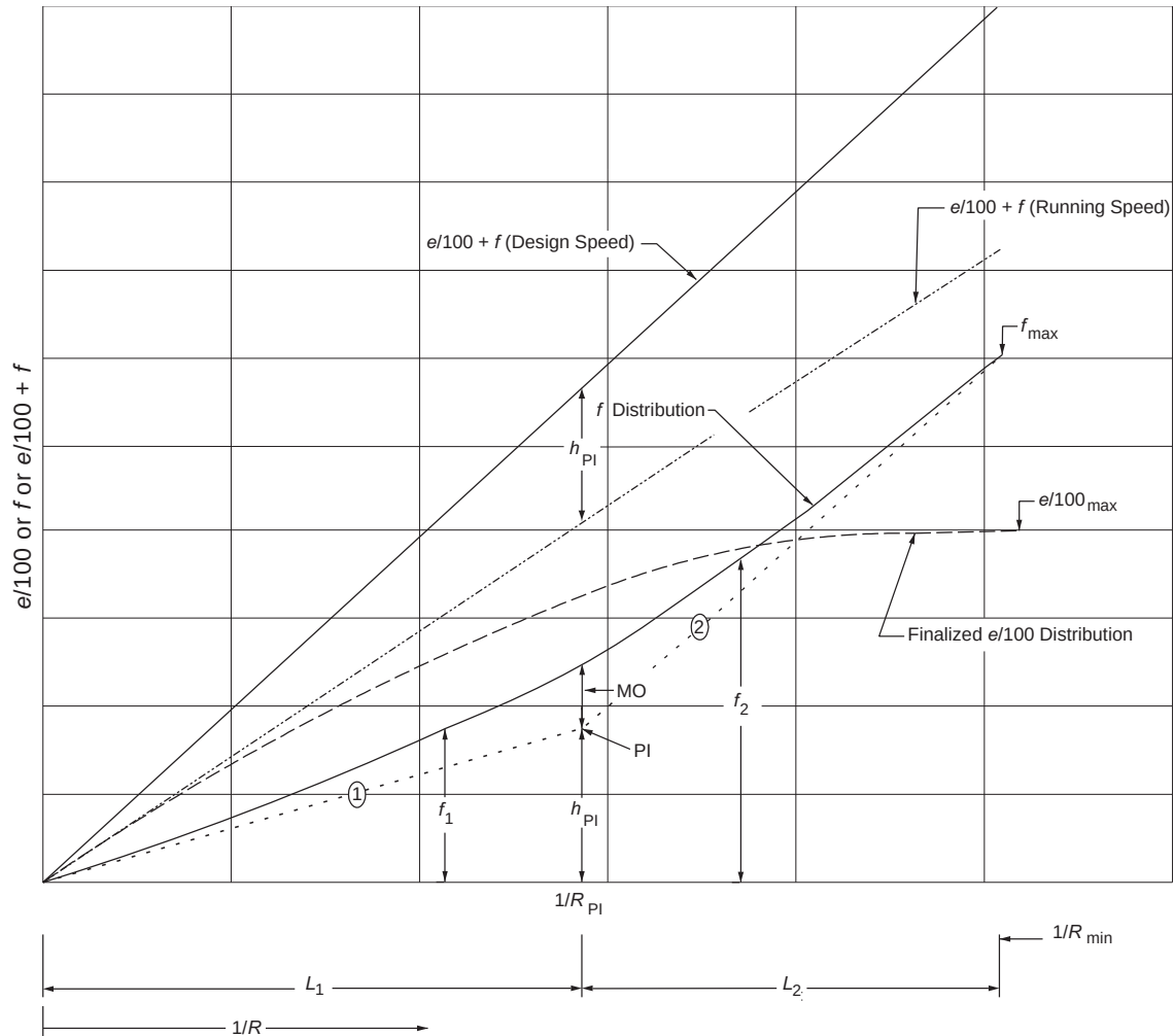
Figure 3-8. Method 5 Procedure for Development of the Superelevation Distribution
