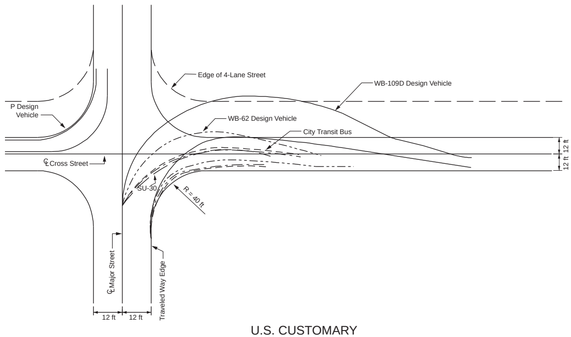
Figure 9-32. Effect of Curb Radii on Right-Turning Paths of Various Design Vehicles
