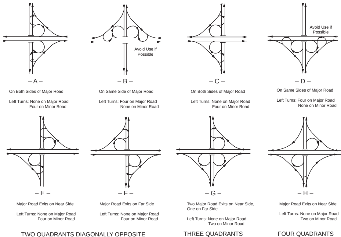
Figure 10-29. Schematic of Partial Cloverleaf Ramp Arrangements, Exit and Entrance Turns
