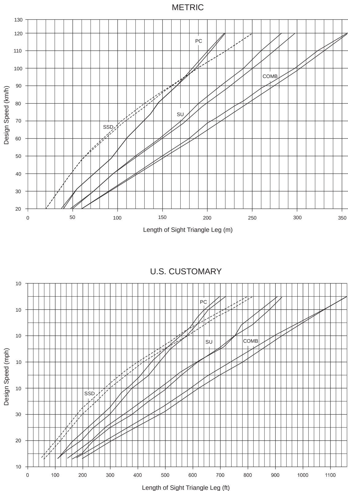
Figure 9-18. Intersection Sight Distance—Case B2, Right Turn from Stop, and Case B3, Crossing Maneuver
