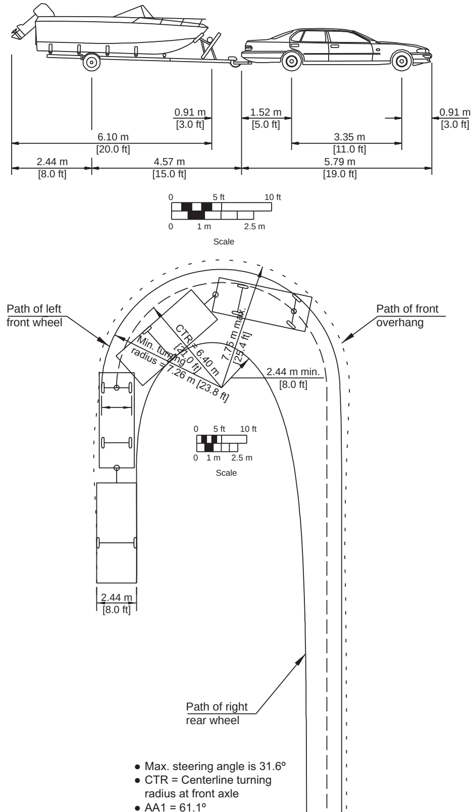
Figure 2-22. Minimum Turning Path for Passenger Car and Boat Trailer (P/B) Design Vehicle
