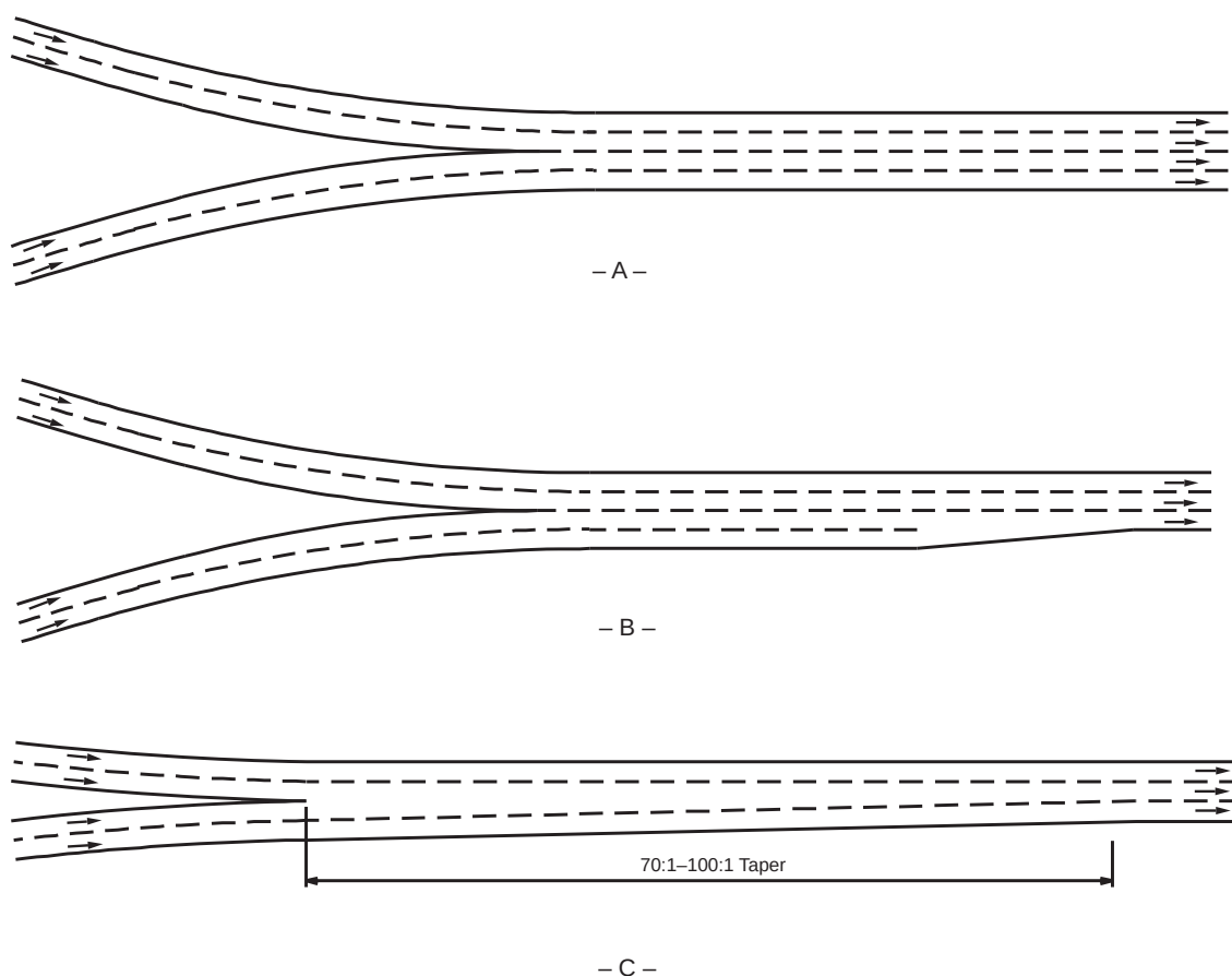
Figure 10-76. Branch Connections
