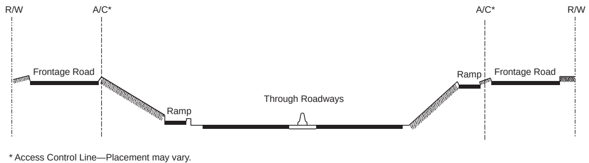
Figure 8-3. Typical Cross Section for Depressed Freeways
