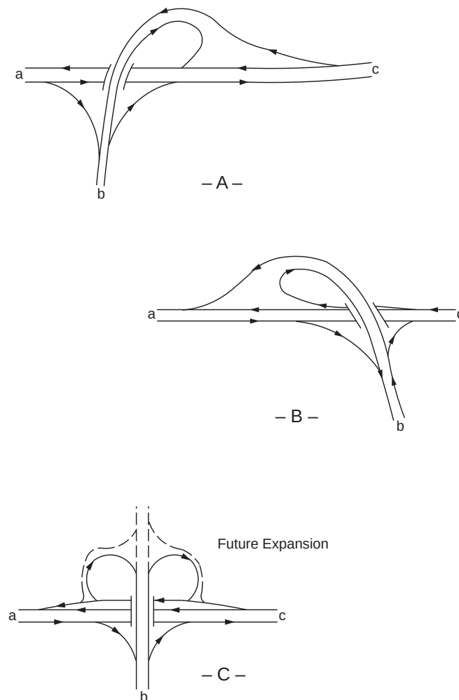
Figure 10-9. Three-Leg Interchanges with Single Structures
