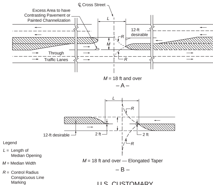
Figure 9-51. Median Left-Turn Design for Median Width in Excess of 5.4 m [18 ft]
