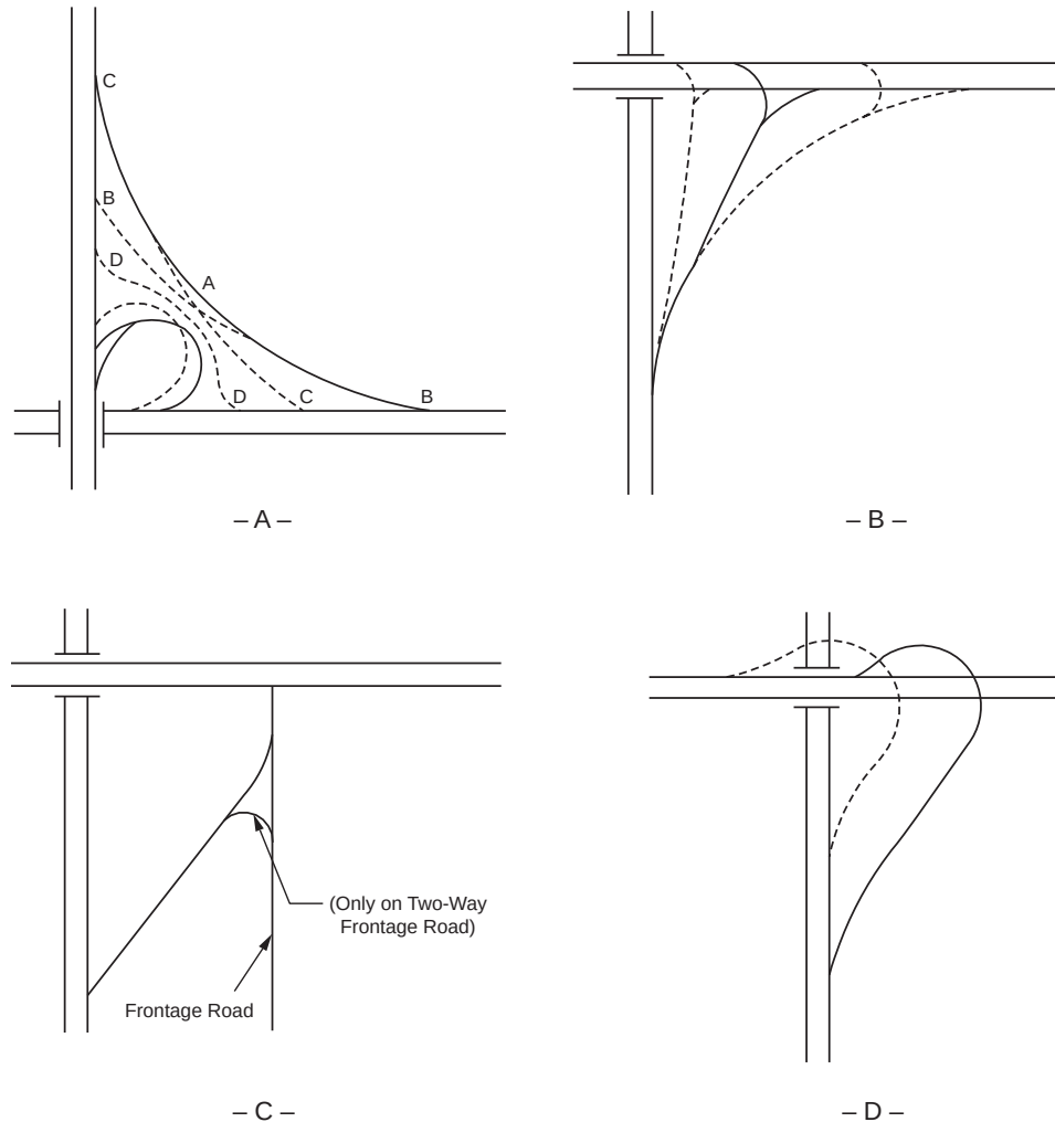
Figure 10-59. Ramp Shapes
