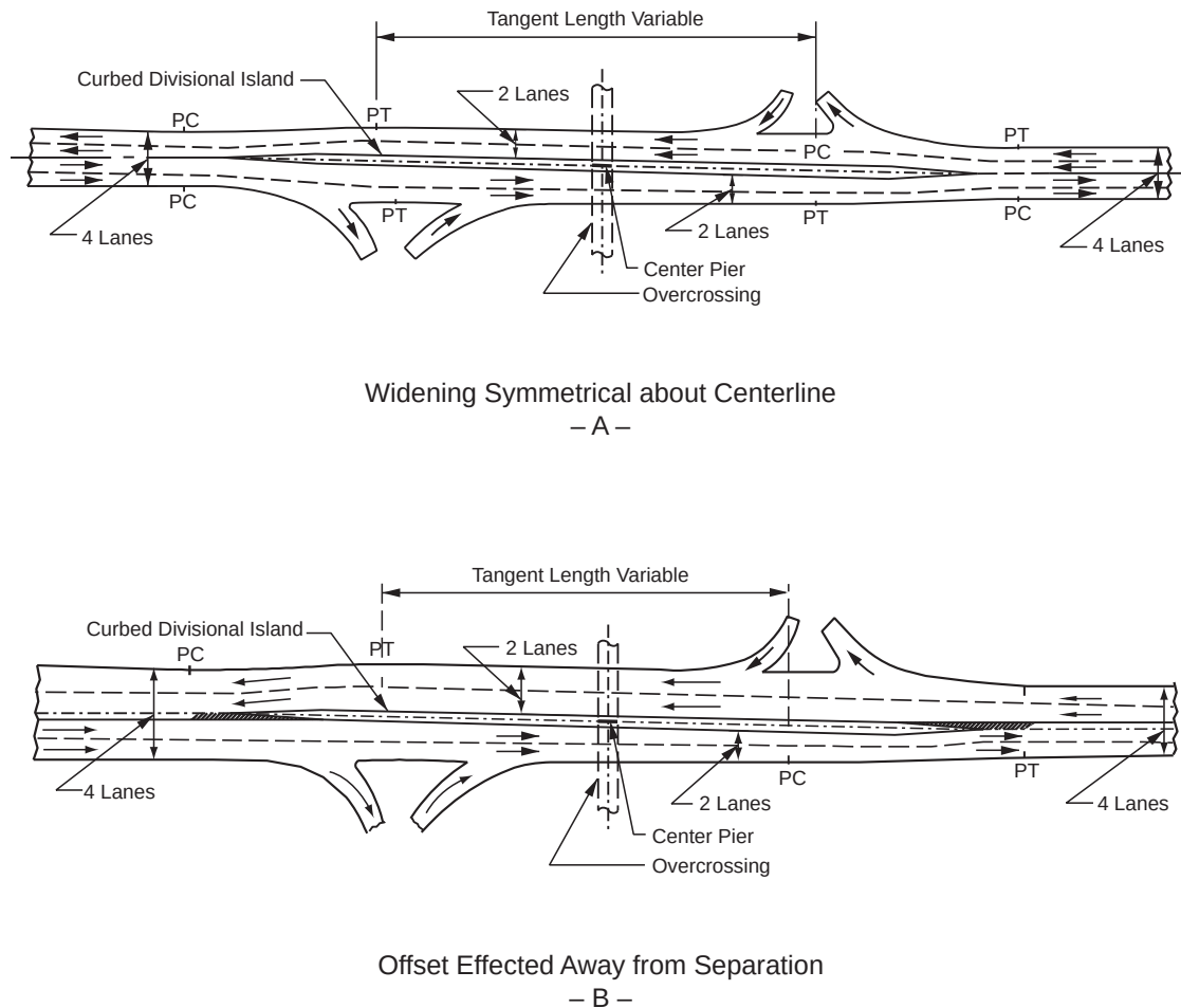
Figure 10-45. Widening for Divisional Island at Interchanges
