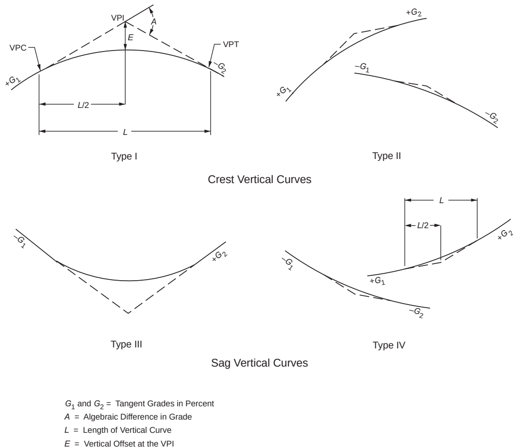
Figure 3-41. Types of Vertical Curves
