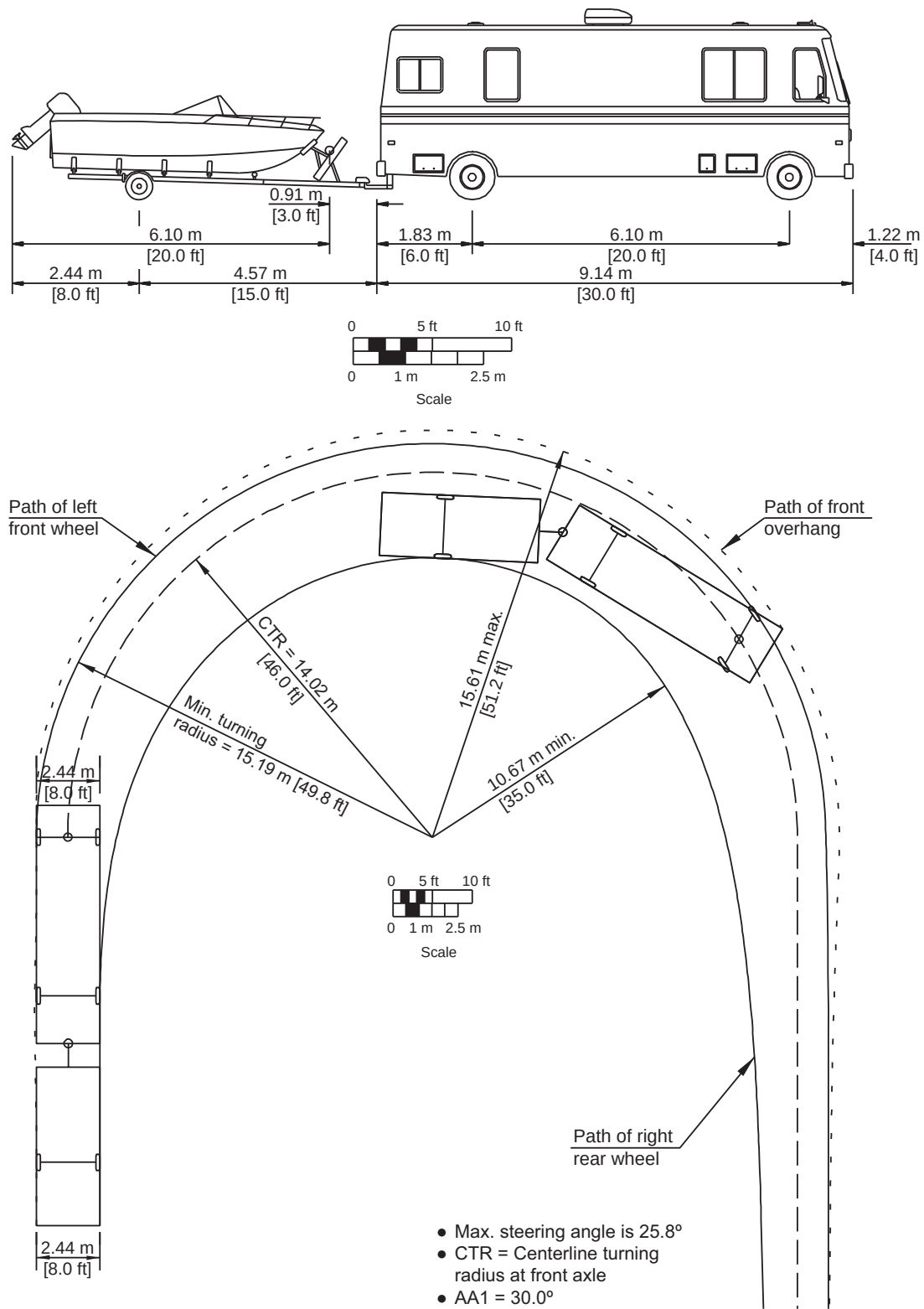
Figure 2-23. Minimum Turning Path for Motor Home and Boat Trailer (MH/B) Design Vehicle
