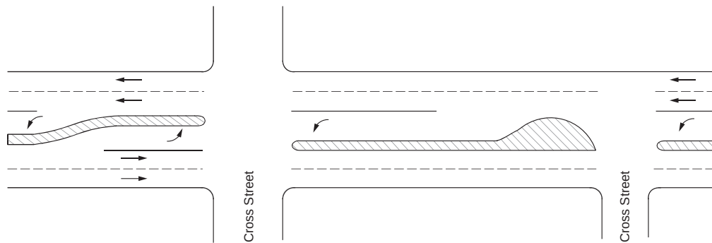
Typical Multilane Highway with Painted Left-Turn Lane Channelization into Cross Streets
