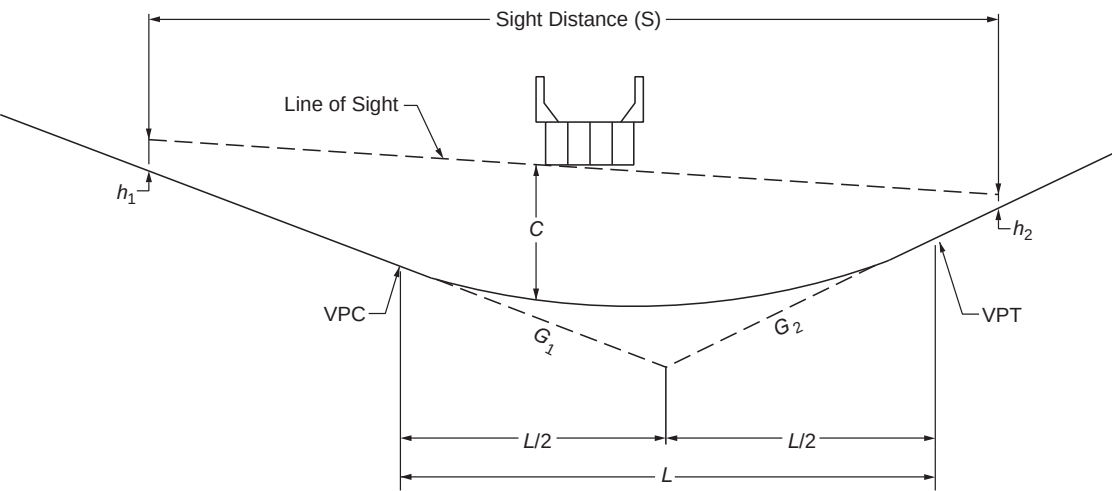
Figure 3-45. Sight Distance at Undercrossings
