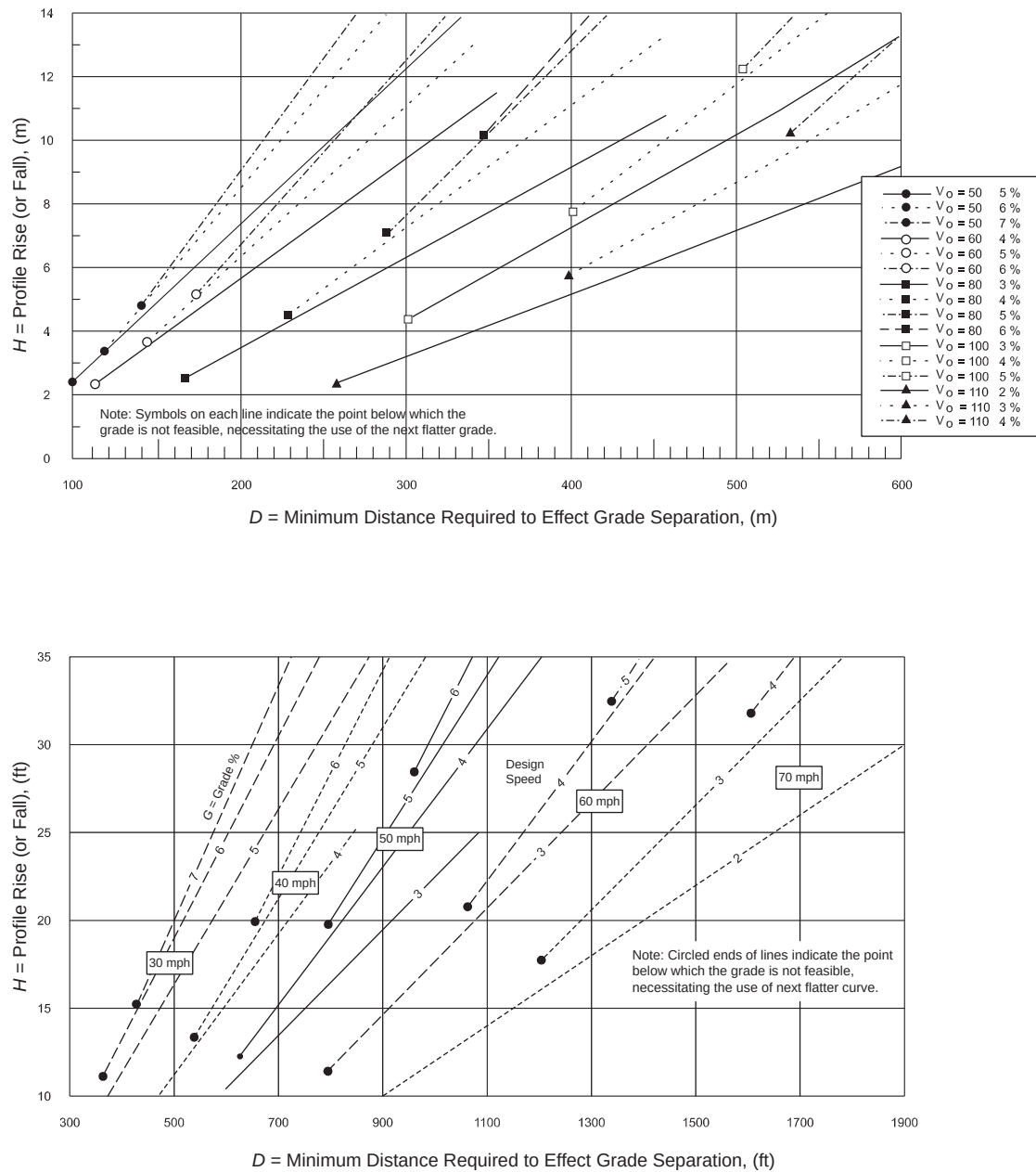
Figure 10-8. Flat Terrain, Distance Needed to Achieve Grade Separation
