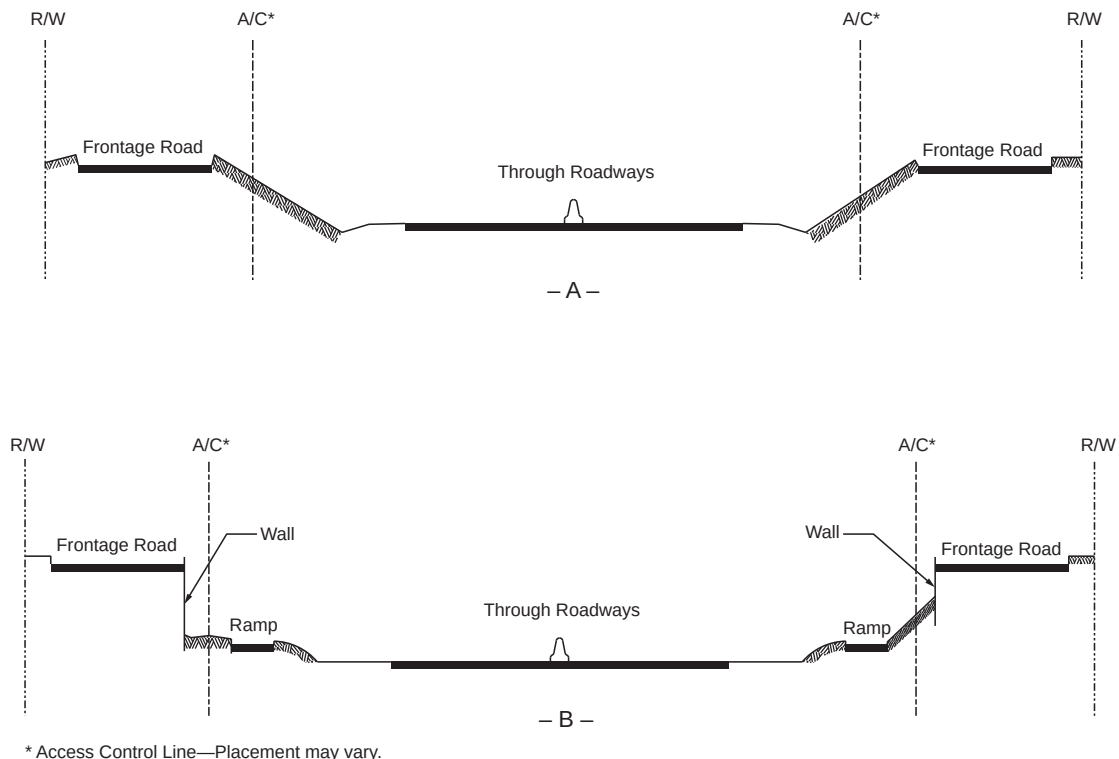
Figure 8-4. Restricted Cross Sections for Depressed Freeways
