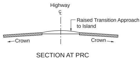
Figure 9-41. Details of Divisional Island Design
