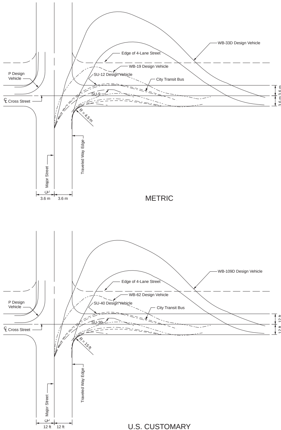
Figure 9-31. Effect of Curb Radii on Right-Turning Paths of Various Design Vehicles
