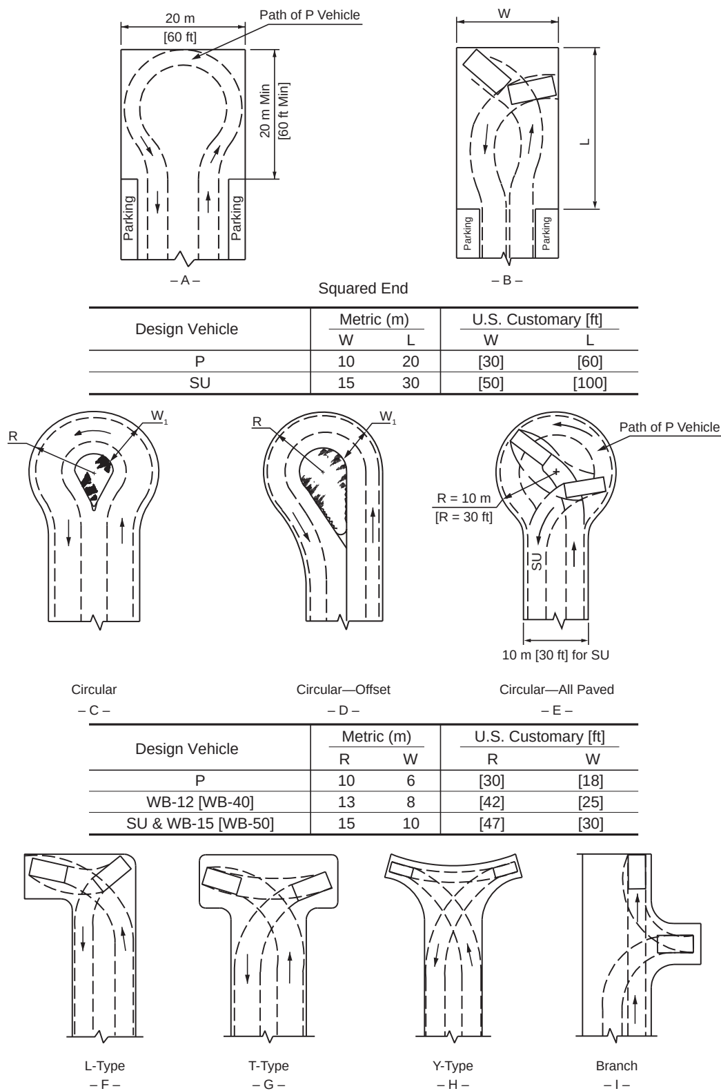
Figure 5-1. Types of Cul-de-Sacs and Dead-End Streets
