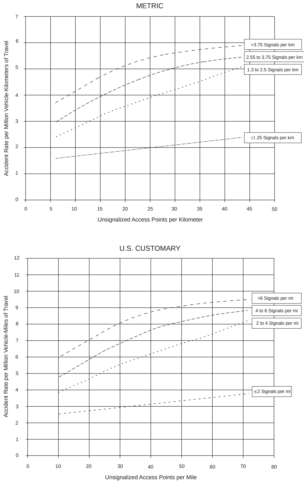
Figure 2-34. Estimated Crash Rates by Unsignalized and Signalized Access Density—Urban and Suburban Areas (22)
