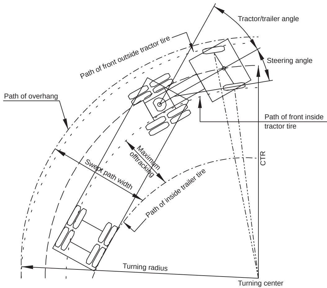
Figure 2-10. Turning Characteristics of a Typical Tractor-Semitrailer Combination Truck
