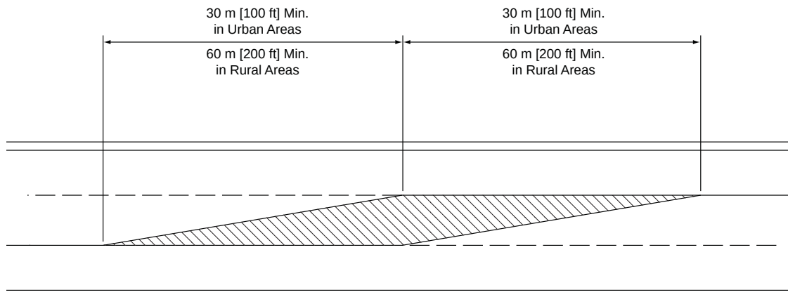
Figure 3-37. Schematic for Adjacent Lane Addition Tapers on a 2+1 Roadway
