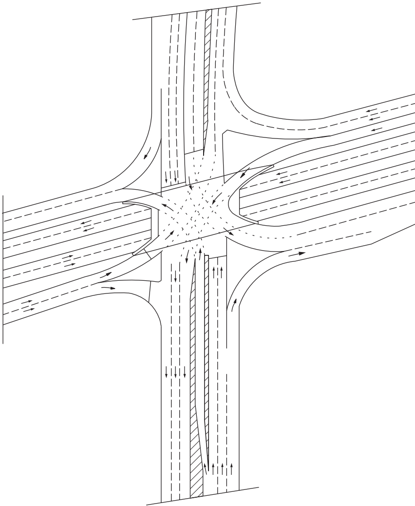
Figure 10-24. Typical SPD Underpass Configuration in Restricted Right-of-Way
