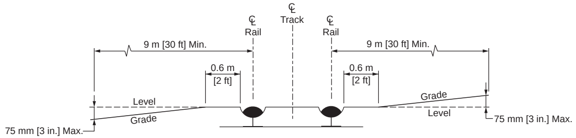
Figure 9-75. Railroad-Highway Grade Crossing
