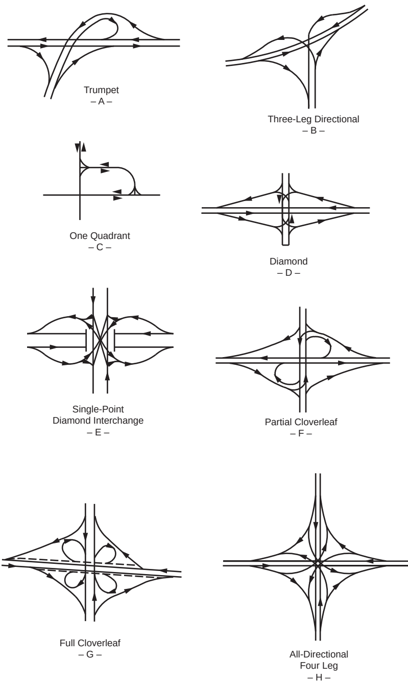
Figure 10-1. Interchange Configurations
