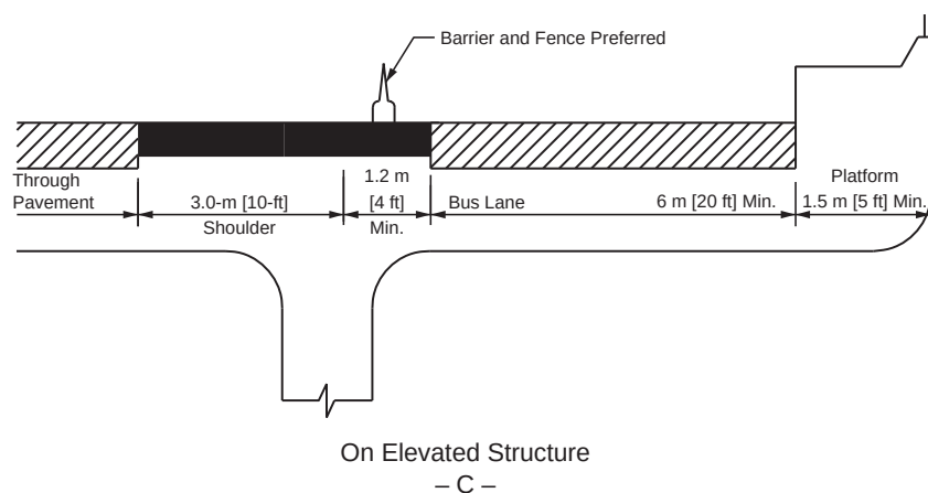
Figure 4-22. Bus Turnouts
