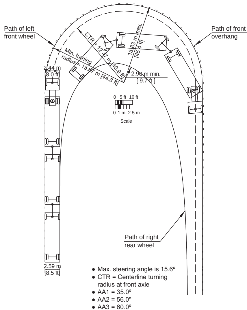
Figure 2-18. Minimum Turning Path for Triple-Trailer Combination (WB-30T [WB-100T]) Design Vehicle
