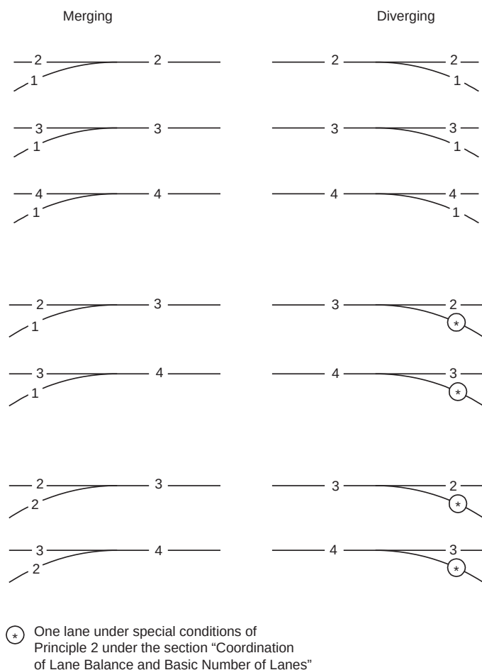
Figure 10-50. Typical Examples of Lane Balance
