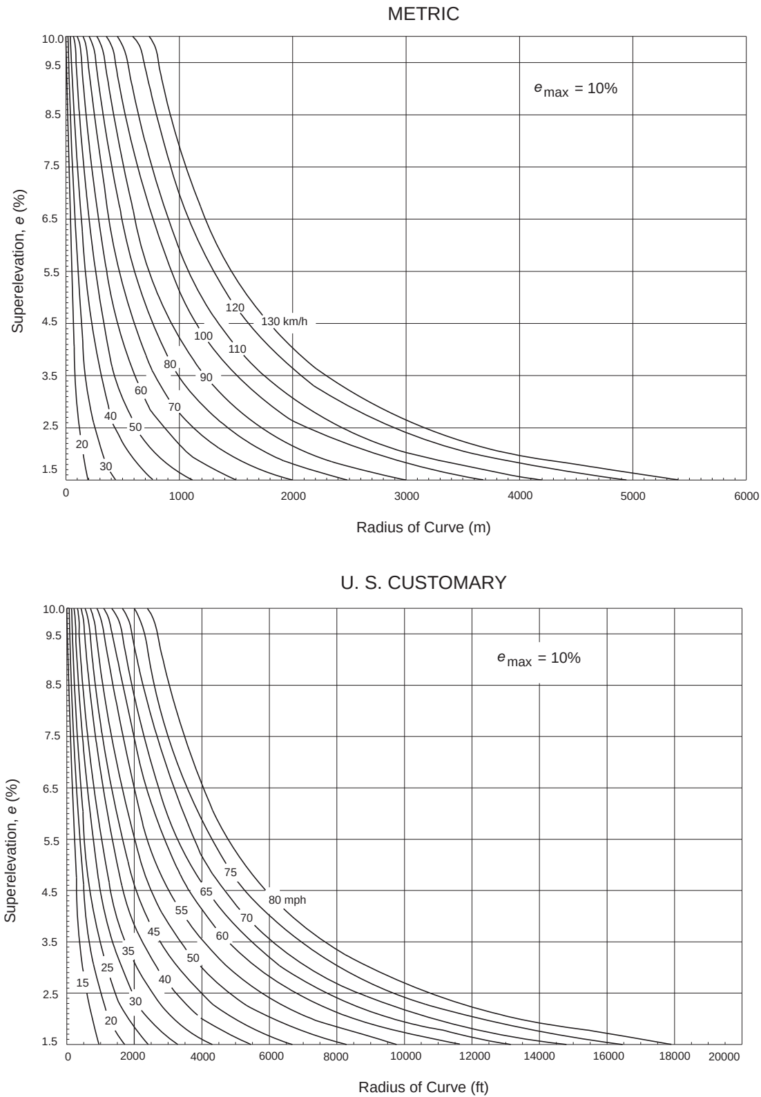
Figure 3-12. Design Superelevation Rates for Maximum Superelevation Rate of 10 Percent
