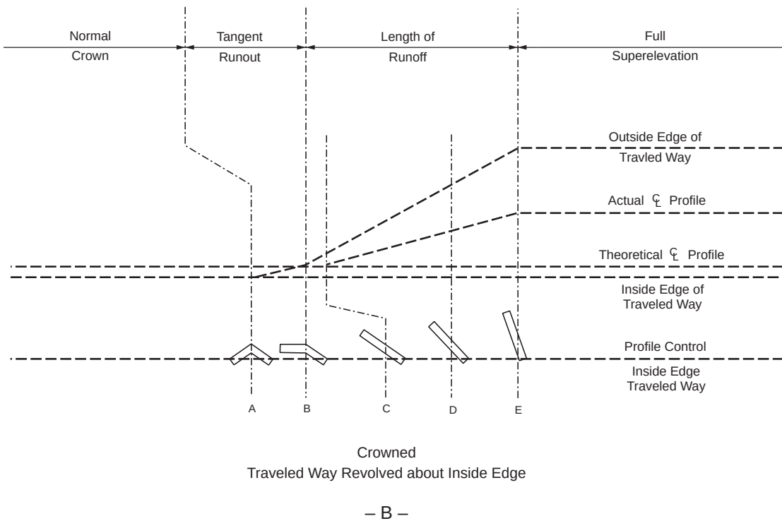
Figure 3-16. Diagrammatic Profiles Showing Methods of Attaining Superelevation for a Curve to the Right
