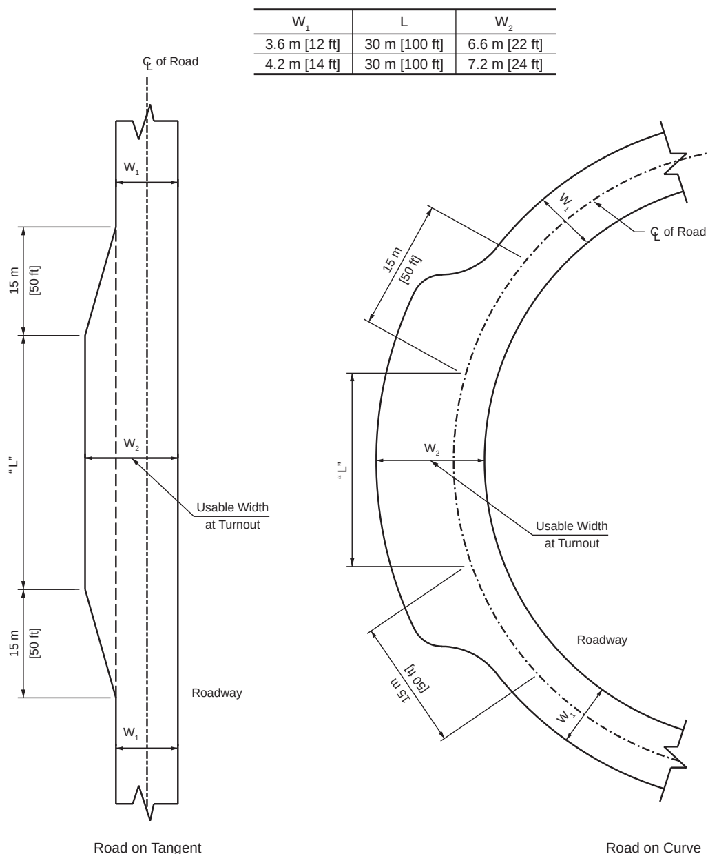
Figure 5-6. Turnout Design
