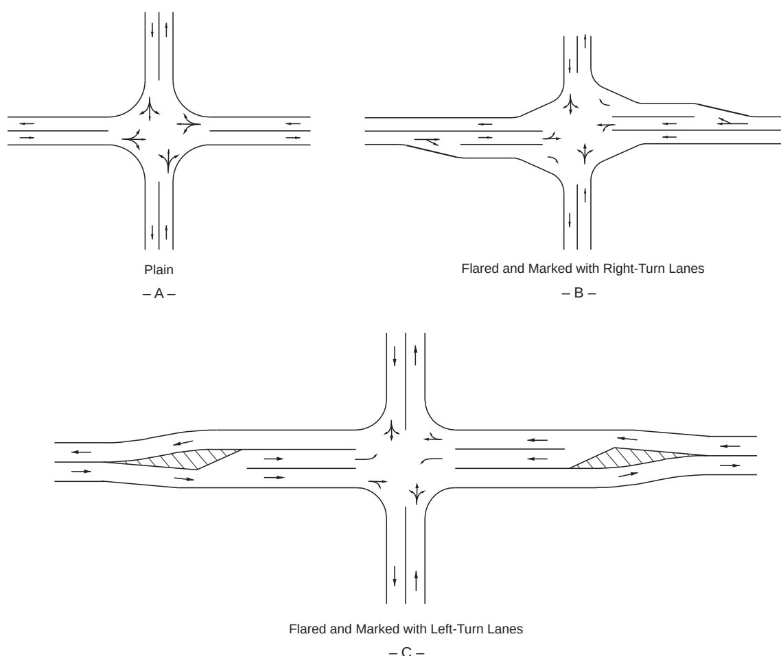
Figure 9-6. Unchannelized Four-Leg Intersections, Plain and Flared
