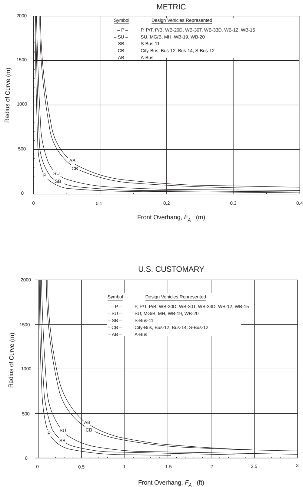
Figure 3-18. Front Overhang for Widening of Traveled Way on Curves
