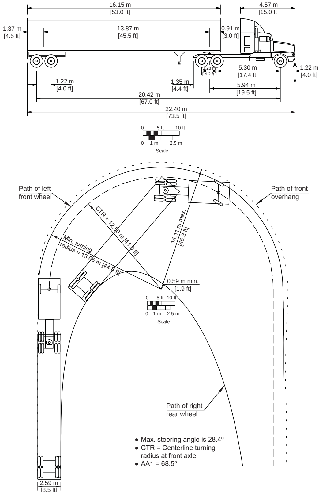
Figure 2-15. Minimum Turning Path for Interstate Semitrailer (WB-20 [WB-67]) Design Vehicle
