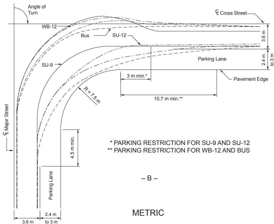
Figure 9-33. Effect of Curb Radii and Parking on Right-Turning Paths
