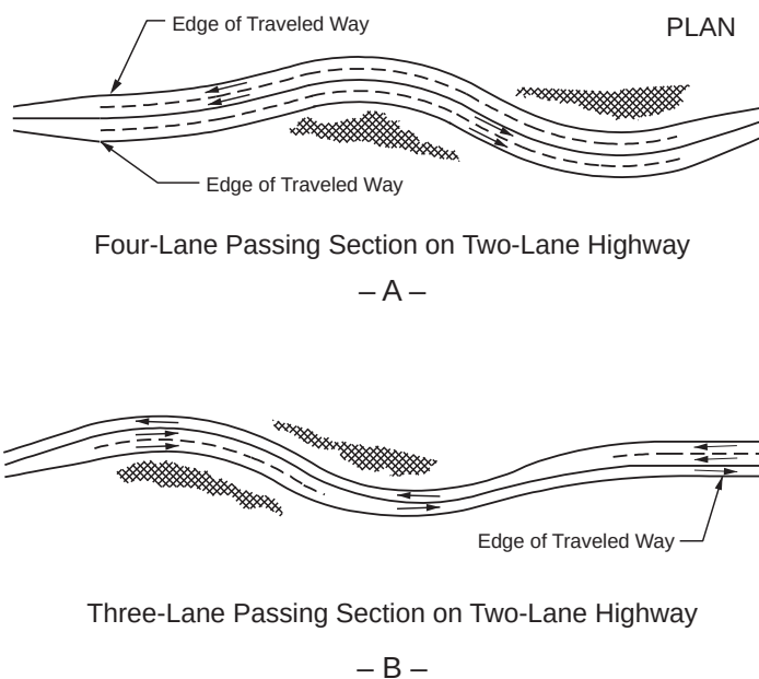
Figure 3-32. Passing Lanes Section on Two-Lane Roads
