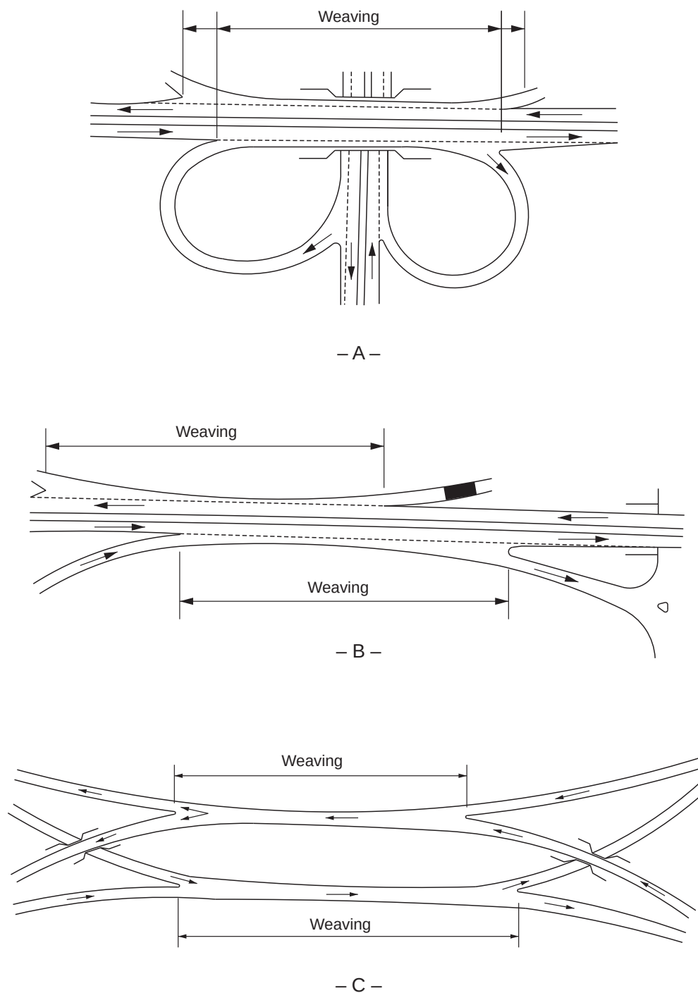
Figure 2-30. Weaving Sections
