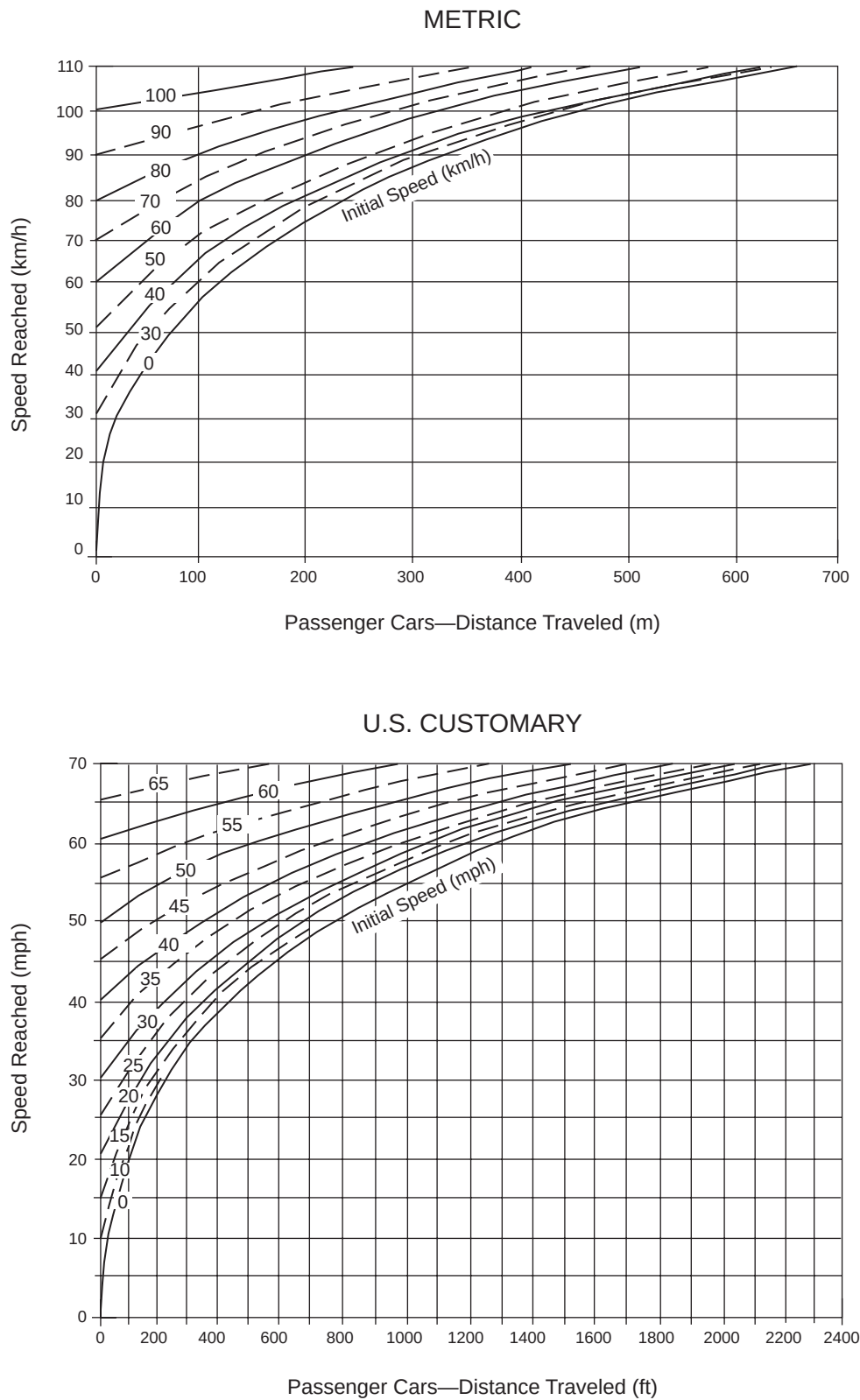
Figure 2-24. Acceleration of Passenger Cars, Level Conditions
